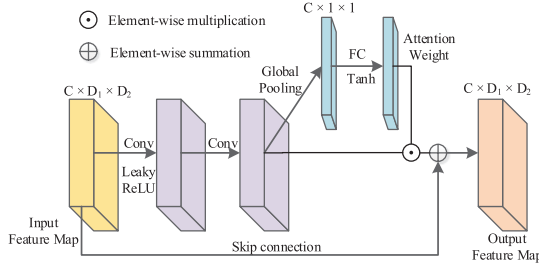
Fig. 3. The improved channel attention block.
