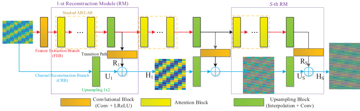
Fig. 4. The proposed Laplacian pyramid attention network (LPAN) architecture.
