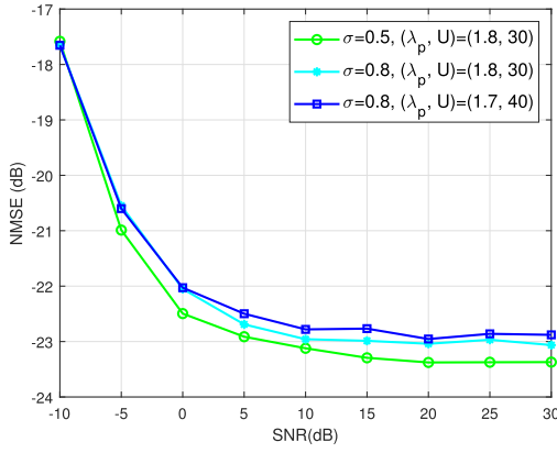
Fig. 14. NMSE performance of LPAN-L under different angular spreads \sigma and scattering distribution (\lambda_p, U) .
