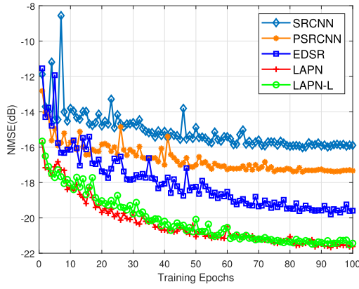
Fig. 8. Convergence performance with training epochs E of DL estimators.
