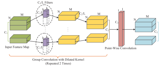
Fig. 5. The proposed lightweight convolution module in LPAN-L.
